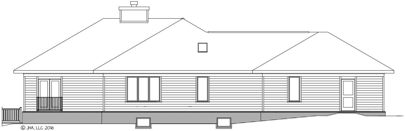
LEFT ELEVATION
