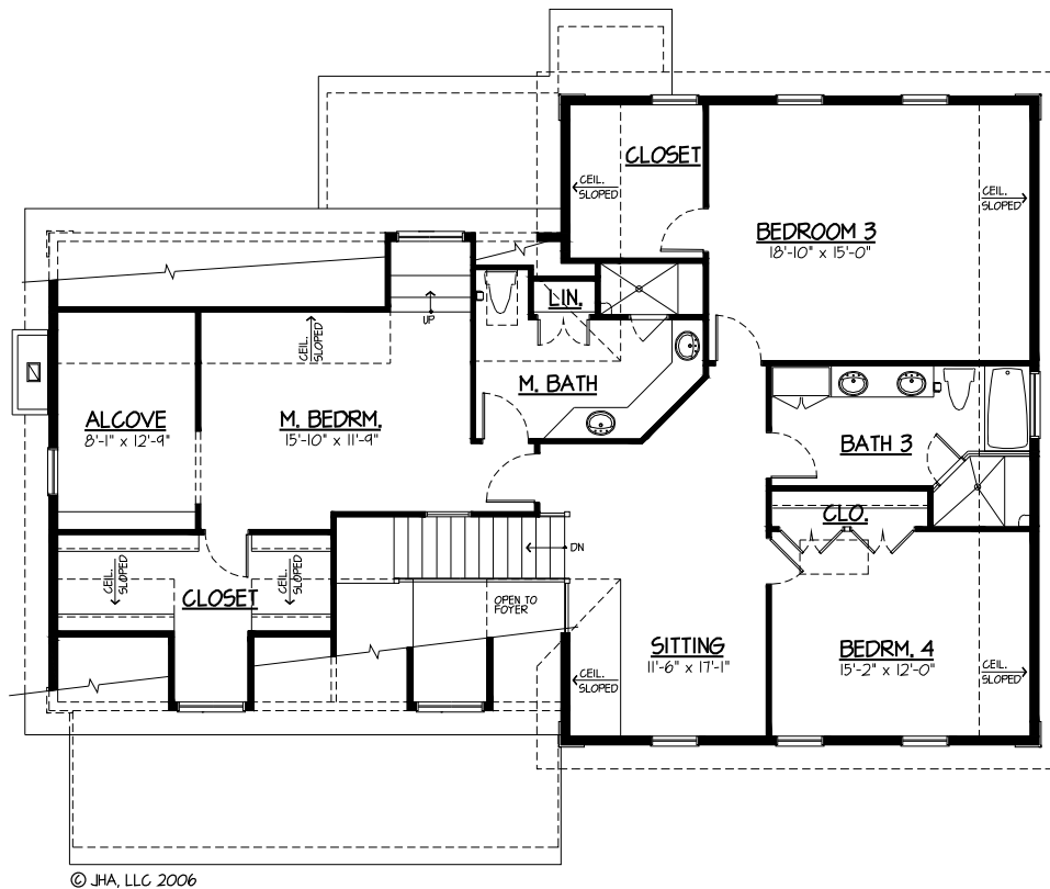
SECOND FLOOR
